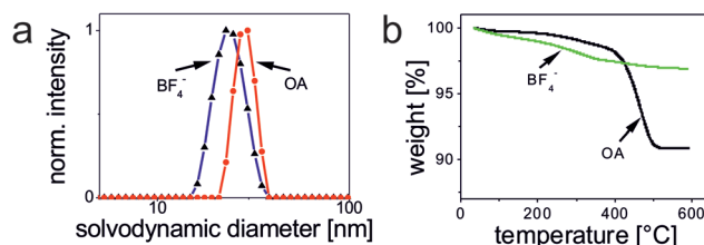
Fig. 3 (a) The solvodynamic diameter (intensity-weighted distribution) of OA-coated UCNPs in cyclohexane is 29 nm (PDI 0.189 ), and 24 nm (PDI 0.089 ) for \text{BF}_4^- -coated UCNPs ( \text{BF}_4^- ) in DMF. (b) TGA experiments quantifying the relative mass loss of OA-coated and \text{BF}_4^- -coated UCNPs as \sim 9.1\% and \sim 3.1\% , respectively.
